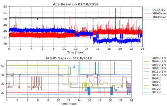
Figure 1: Electron beam size as measured the ALS diagnostic beamline 3.1 during a user run (top) showing roughly 2.5 μm variation (5%) in the vertical caused by changes in vertical ID gaps (shown, bottom) and horizontal EPU shifts (not shown here).
